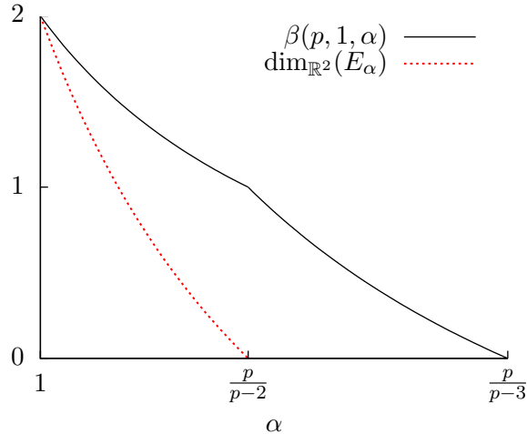
FIGURE 2. The quantity \beta(p, 1, \alpha) of Theorem 1.5 and the dimension of the set E_\alpha of Theorem 1.9.
