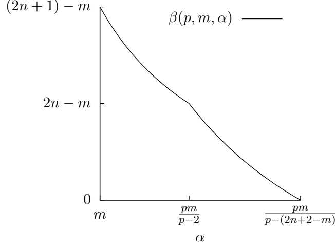
FIGURE 1. The quantity \beta(p, m, \alpha) of Theorem 1.5 as a function of \alpha .
